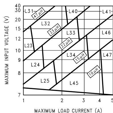
Figure 22. LM2678-5.0
